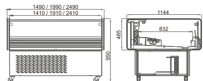
Luxury air-cooled open fresh meat display case
