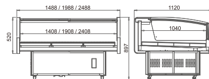
Direct Cooling Glass Door Meat Display Case
