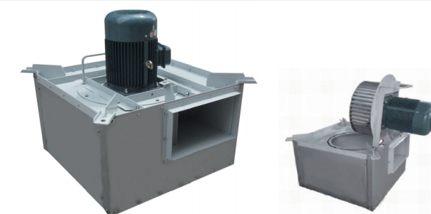
Exhausted Fan13-48-R3-DG
